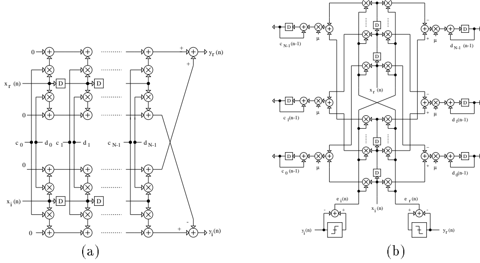
Figure 23: The crosscoupled equalizer structure: (a) the \mathbf{F} block and, the (b) \mathbf{WUD} block.
