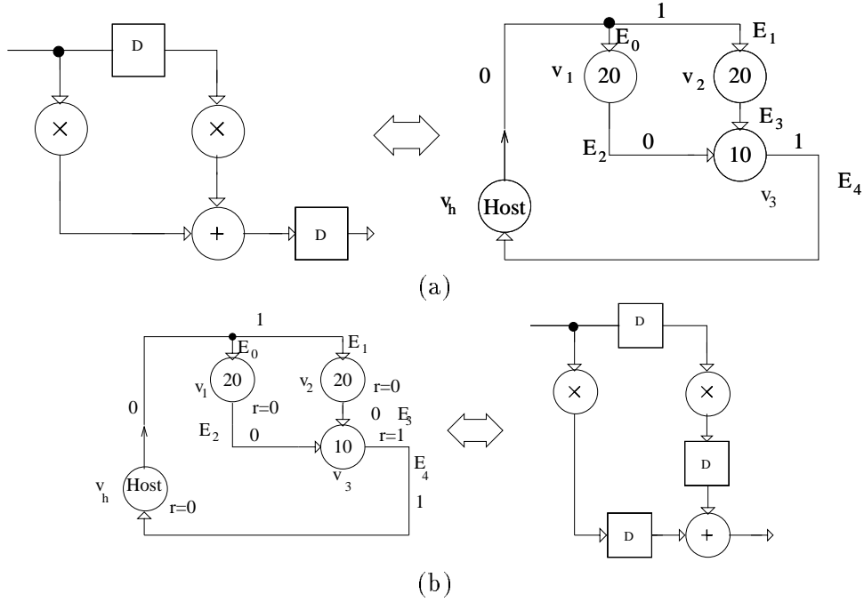
Figure 7: An systematic retiming example:(a) the original DFG and (b) the retimed DFG.
