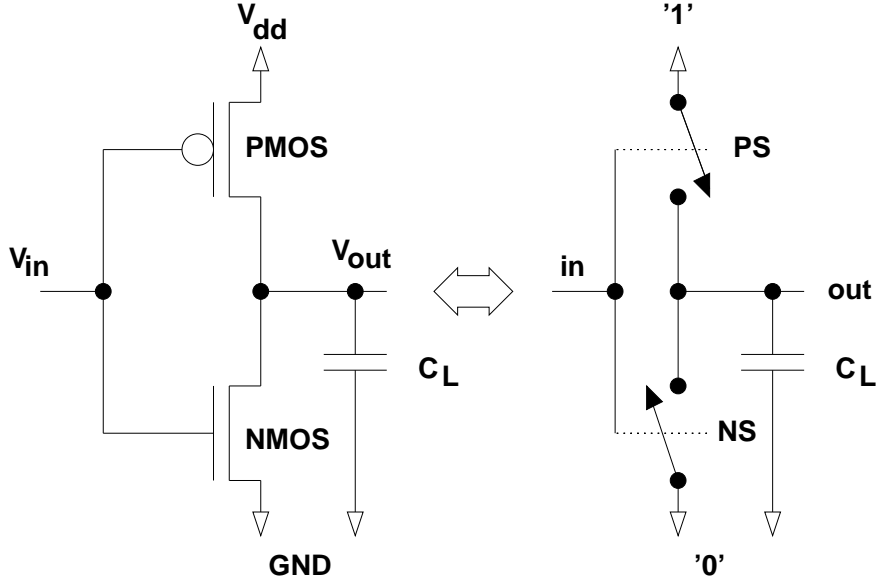
Figure 4: Power dissipation in CMOS circuits.
