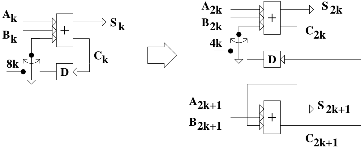
Figure 19: Unfolding of a bit-serial adder.
