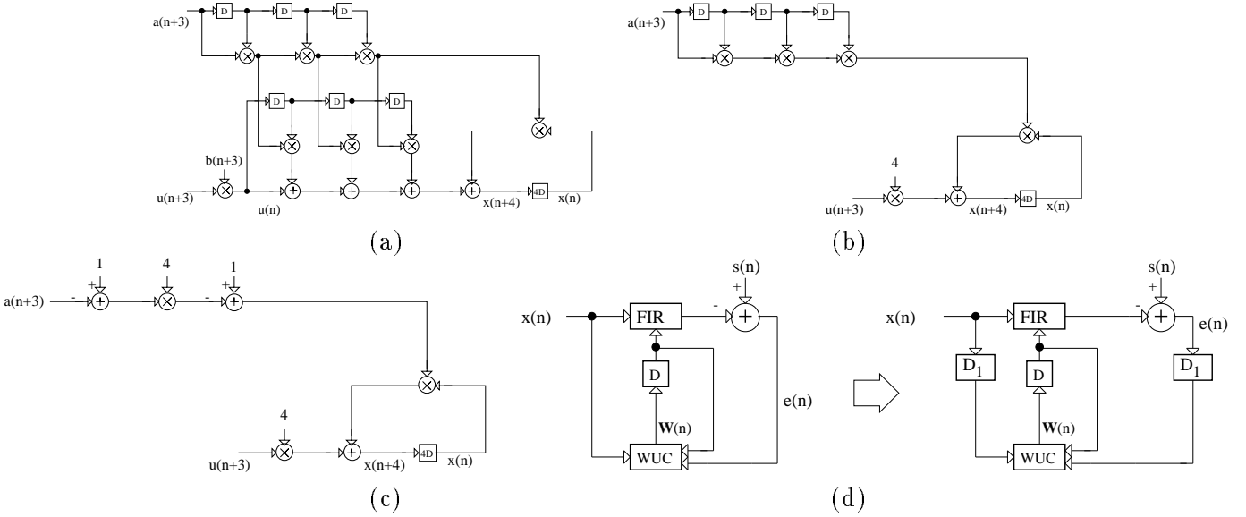
Figure 14: Relaxed look-ahead pipelining: (a) look-ahead pipelining, (b) sum, (c) product, and (d) delay relaxations.
