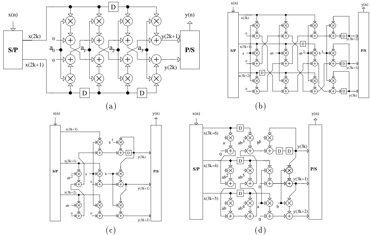
Figure 17: Parallel architectures: (a) a parallel FIR filter with L = 2 , N = 3 , (b) a parallel direct form block IIR filter with L = 3 , N = 1 , (c) an incremental parallel direct form IIR filter with L = 3 , N = 1 , and (d) a pipelined incremental parallel direct form IIR filter with L = 3 , N = 1 and M = 2 .
