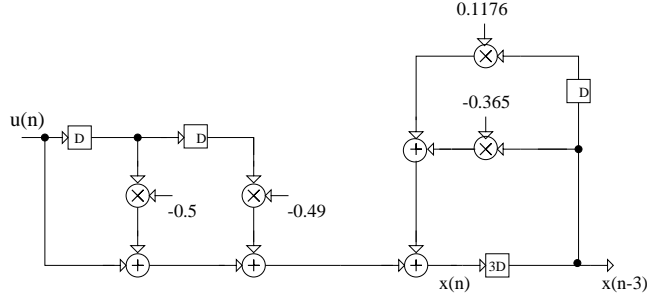
Figure 11: A clustered look-ahead pipelined section.
