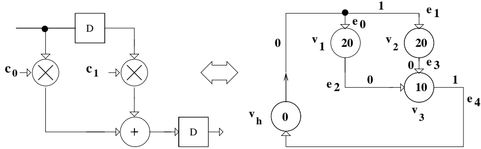
Figure 3: Example of a DFG representation of an FIR filter.
