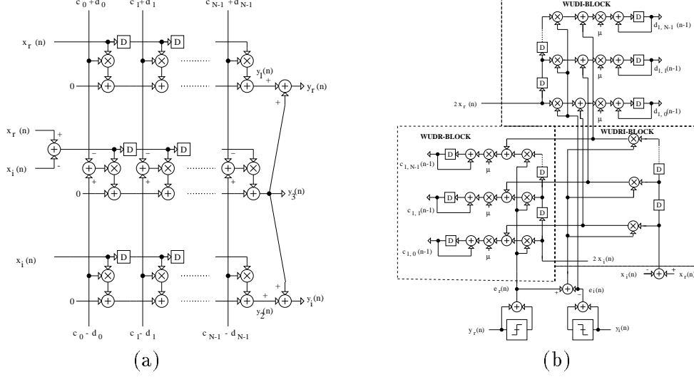
Figure 24: The strength reduced equalizer structure: (a) the F block and, the (b) WUD block.
