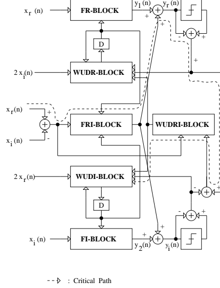
Figure 25: The strength reduced equalizer block diagram.
