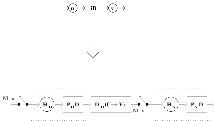
Figure 21: The folding equation.
