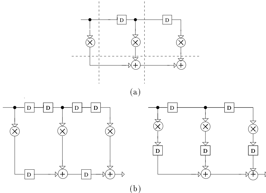
Figure 8: Feedforward cutset pipelining: (a) identification of feedforward cutsets and (b) pipelining via delay placement at the cutsets.
