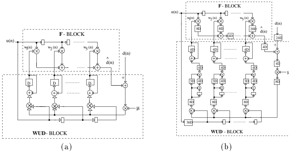
Figure 15: Example: (a) serial architecture and (b) pipelined architecture with speed-up of 48.
