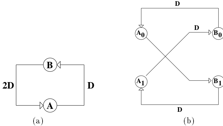
Figure 18: Unfolding transformation: (a) the original DFG, and a (b) 2-unfolded DFG.
