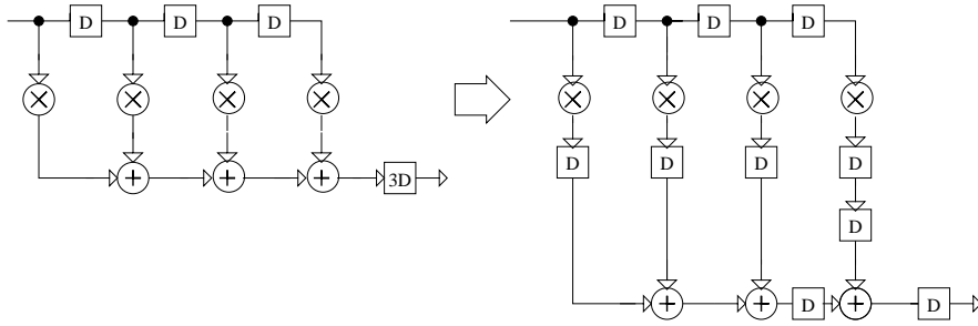
Figure 6: An ad-hoc retiming example.
