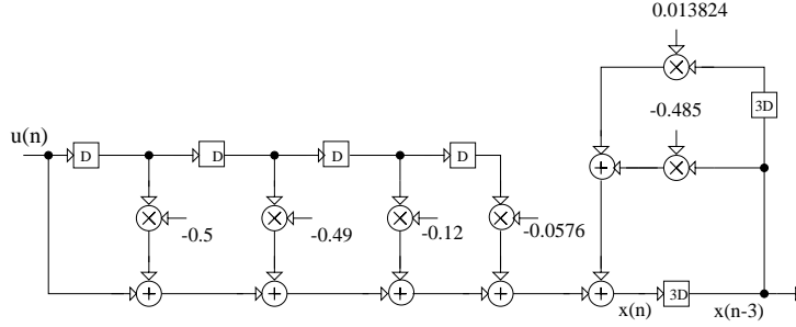
Figure 12: A scattered look-ahead section.
