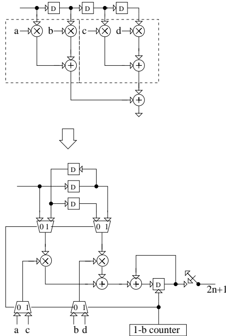
Figure 22: Example of folding.
