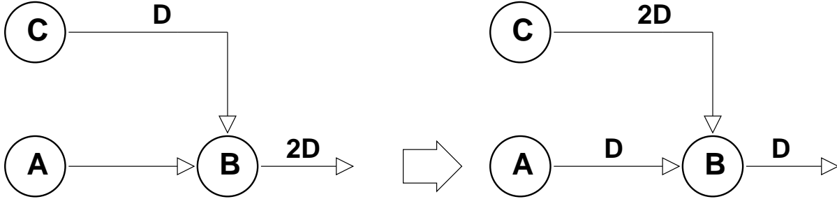
Figure 5: Retiming.
