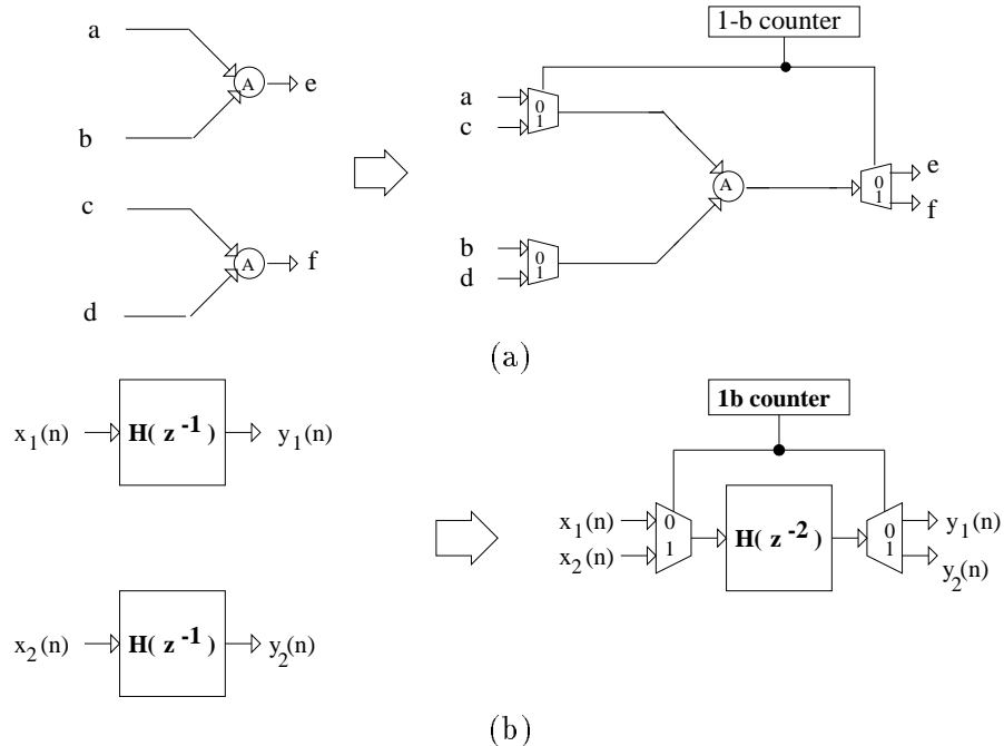
Figure 20: Folding of independent data streams: (a) a general example, and (b) a filter.
