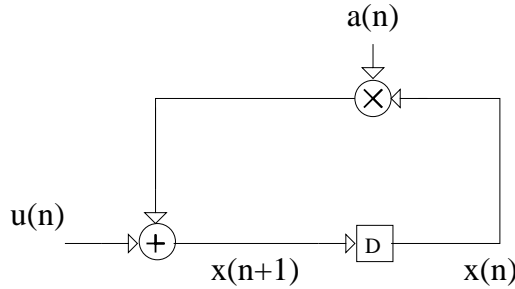
Figure 13: A first order time-varying filter.
