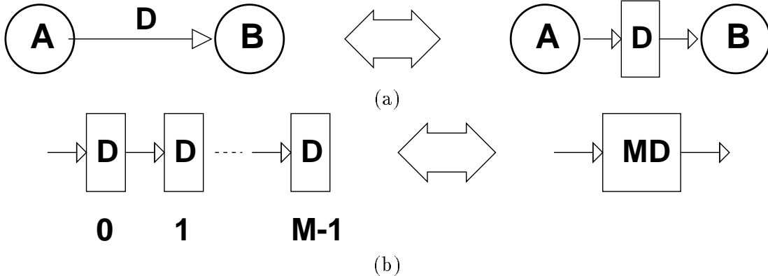
Figure 2: Data-Flow graph representation: (a) alternative DFG representations, and (b) the lumped delay model.
