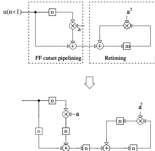
Figure 10: A look-ahead pipelined first-order recursive section.
